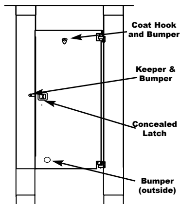
FIGURE 9 (inside view)
